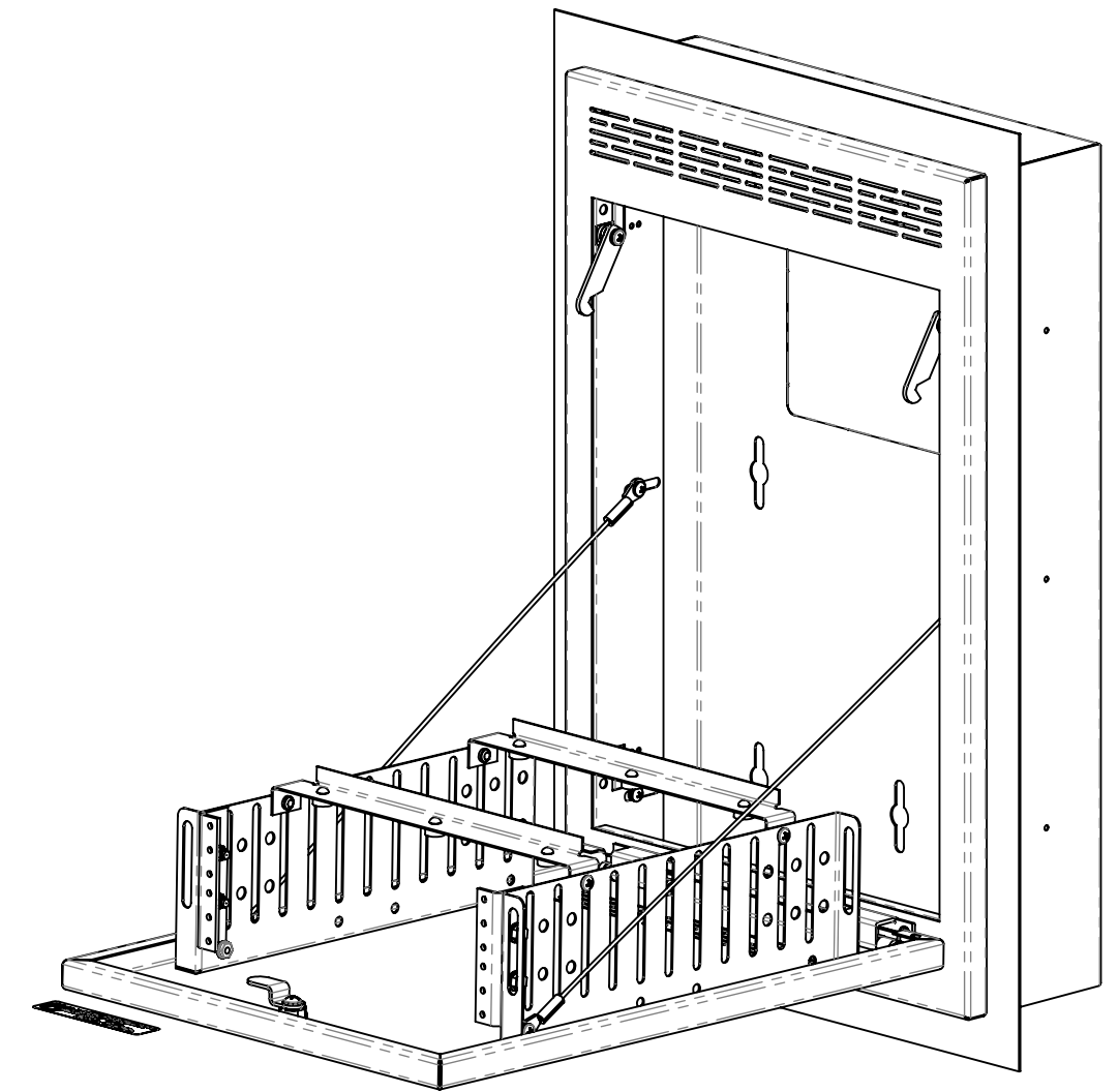
DIMETRIC VIEW DOOR OPEN
